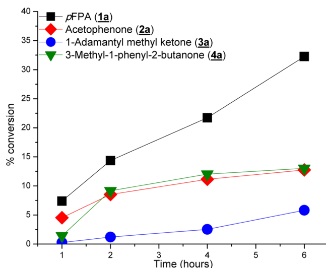
Figure 4. Percent conversion over time in a biphasic organic solvent reaction system. Reaction conditions for p FPA (1 mL): c(pFPA) = 150 mM, c(NADH/NAD^+) = 1 mM, 0.1 mg F-AmDH, V_{organic}/V_{aqueous} = 0.25 , buffer: NH_4HCO_2/OH (5 M, pH 9.6), T = 35 °C. Reaction conditions for 3-methyl-1-phenyl-2-butanone are the same as p FPA. Reaction conditions for acetophenone (1 mL): c(acetophenone) = 150 mM, c(NADH/NAD^+) = 1 mM, 0.25 mg cFL1-AmDH, V_{organic}/V_{aqueous} = 0.25 , buffer: NH_4HCl/OH (5 M, pH 9.6), T = 50 °C. Reaction conditions for 1-adamantyl methyl ketone are the same as acetophenone. All reactions performed with heptane as the organic solvent.
