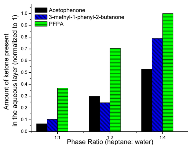
Figure 2. Amount of hydrophobic substrates in the aqueous layer as a function of phase ratio (normalized to 1a , the amount of p FPA in the aqueous phase).
