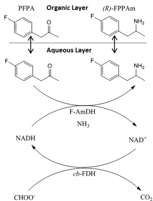
Scheme 1. Biphasic System Reaction Involving F-AmDH and p FPA
